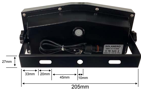
← DIMENSIONS OF BRACKET FOR INSTALL
